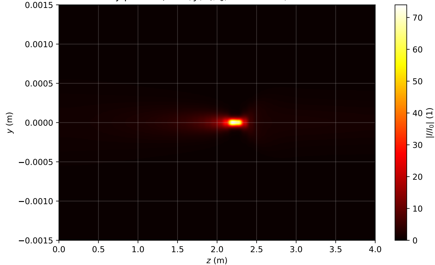
Intensity profile I(x=0, y, z)/I_0 , P_{in}=1.3P_{cr} , artificial time
